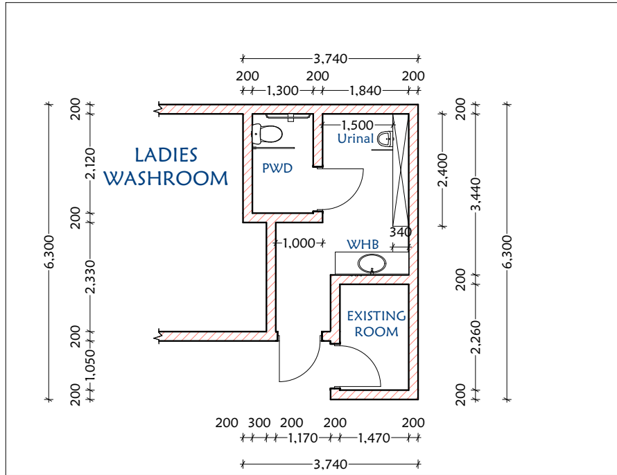
EXISTING MALE WASHROOM GROUND FLOOR, BANKING WING
