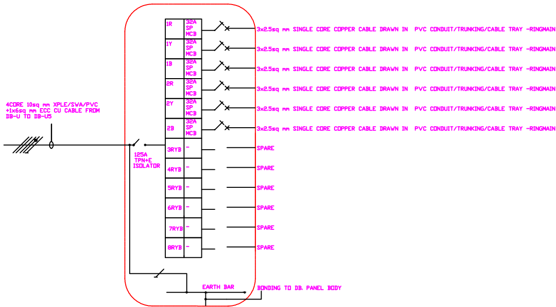
8 WAYS 125A TPN FLUSH MOUNTED DISTRIBUTION BOARD COMPLETE WITH FRONT LATCHED COVER AS DB-U5
