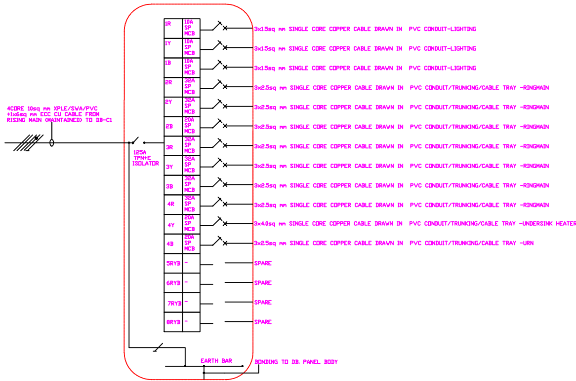
8 WAYS 125A TPN FLUSH MOUNTED DISTRIBUTION BOARD COMPLETE WITH FRONT LATCHED COVER AS DB-C1
