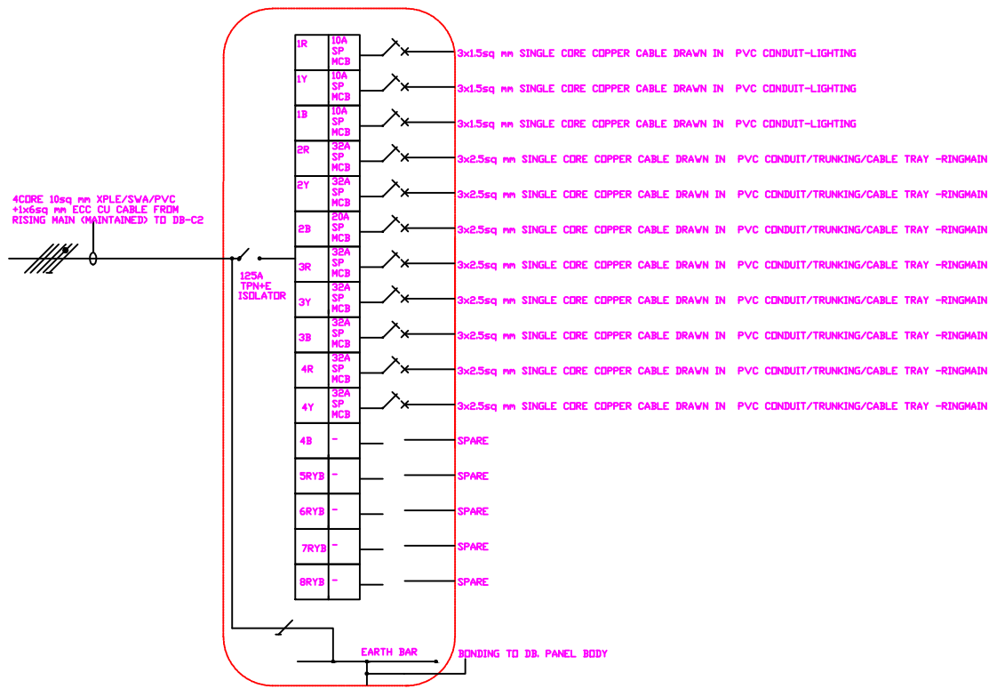
8 WAYS 125A TPN FLUSH MOUNTED DISTRIBUTION BOARD COMPLETE WITH FRONT LATCHED COVER AS DB-C2
