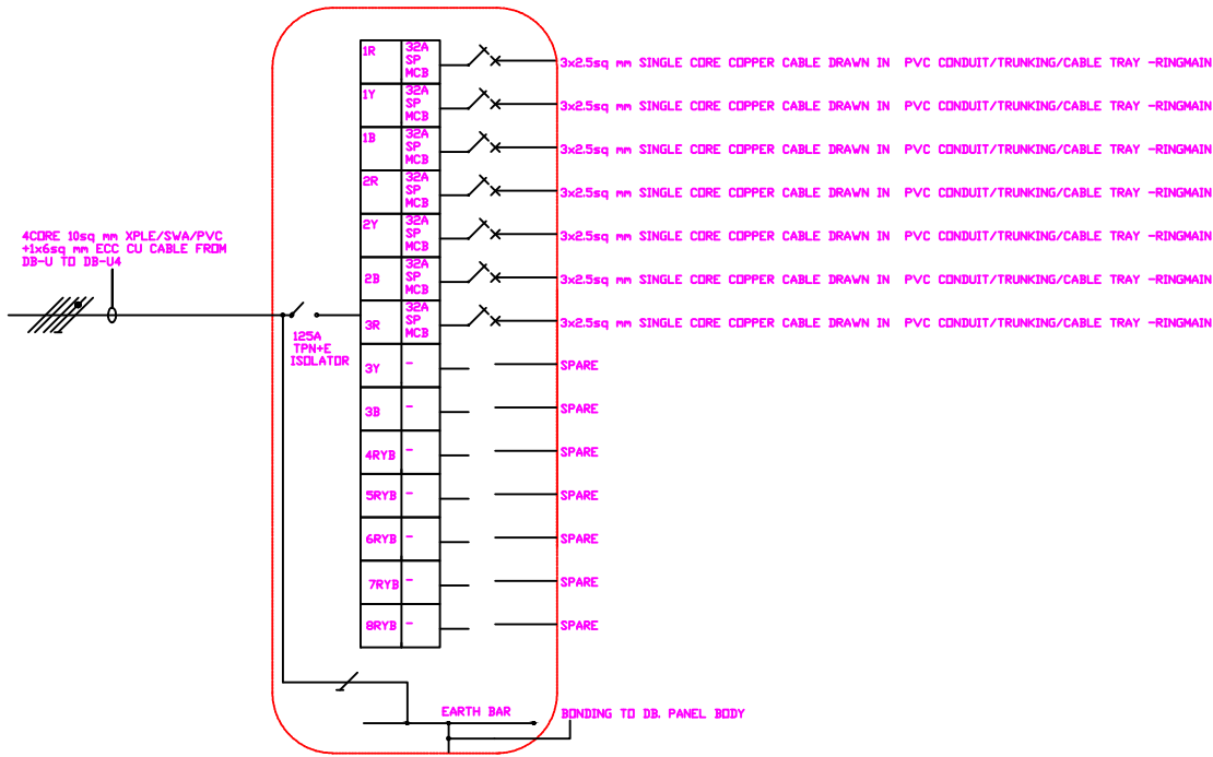
8 WAYS 125A TPN FLUSH MOUNTED DISTRIBUTION BOARD COMPLETE WITH FRONT LATCHED COVER AS DB-U4
