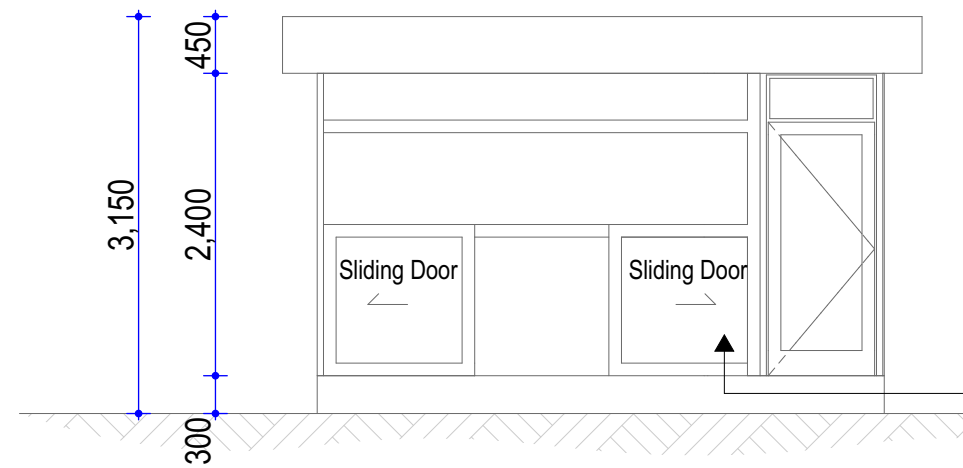
Elevation Two
