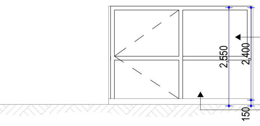
Elevation Two
