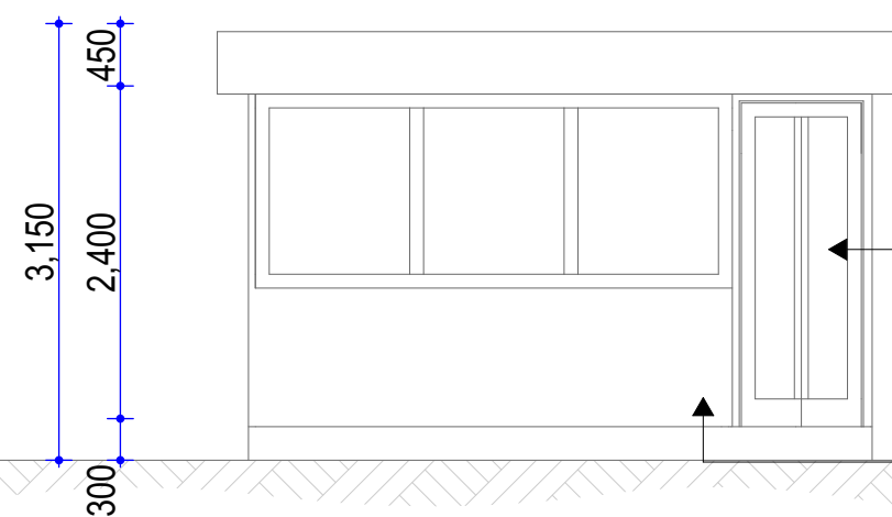
Elevation Four
