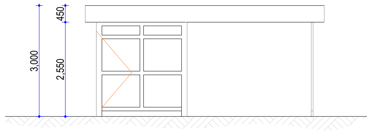
Elevation One
