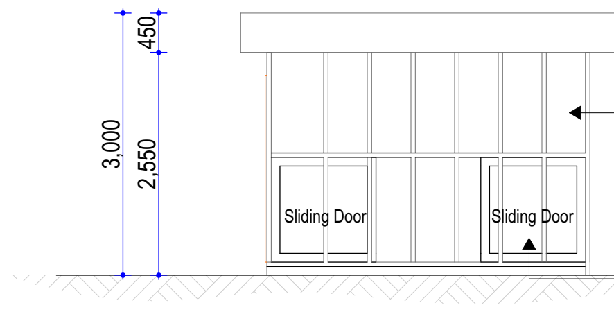
Elevation Two
